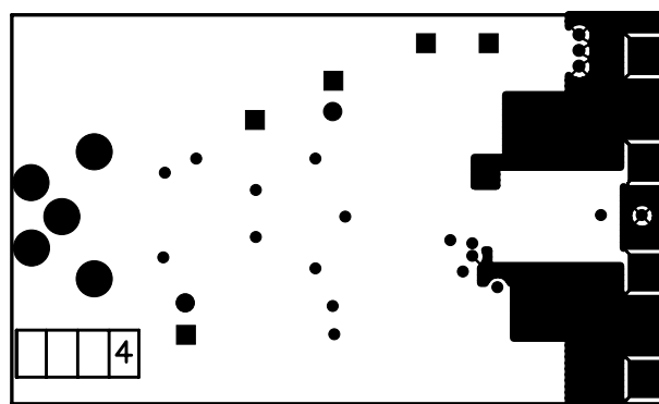
Fig. 33 Bottom Layer of EB1504/08 PCB Layout
