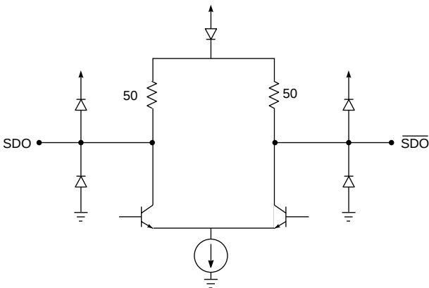
Fig. 4 Output Circuit
