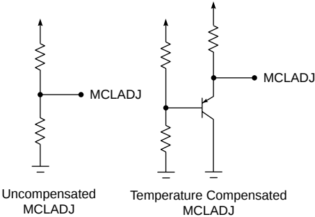
Fig. 10 Temperature Compensation of MCLADJ
