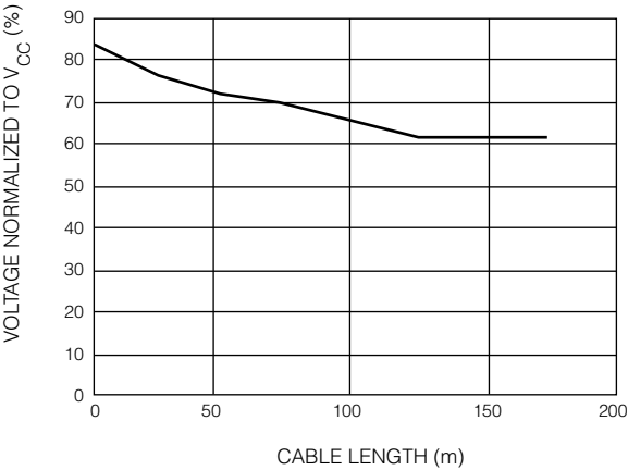
Fig. 12 MCLADJ Input Voltage vs 1694A Cable Length
