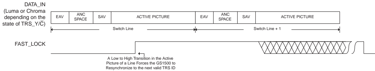
Fig. 5 FAST_LOCK Timing
