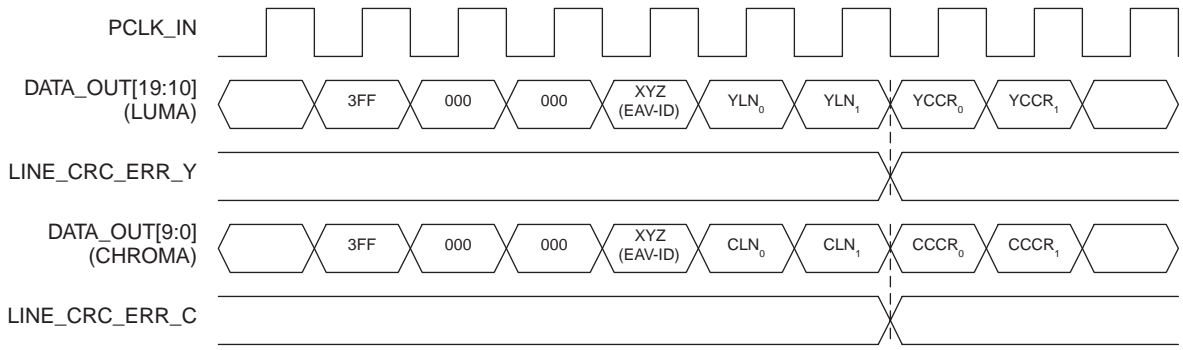
Fig. 6 Luma and Chroma LINE_CRC_ERR Timing
