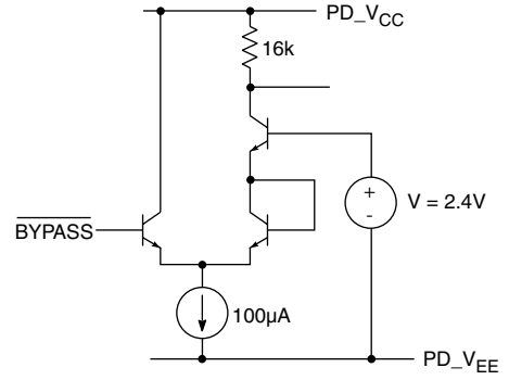
Fig. 10 BYPASS Circuit
