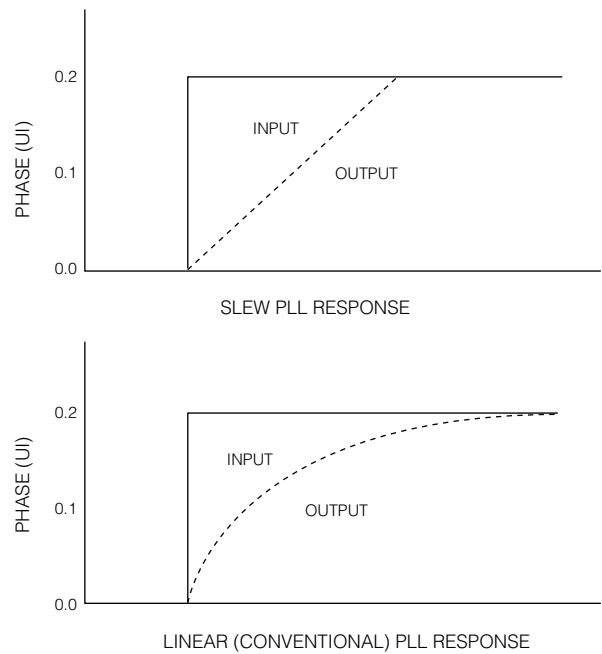
Fig. 16 PLL Characteristics
