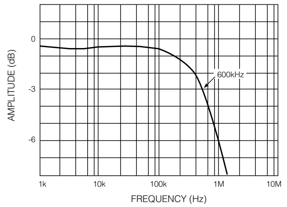
Fig. 13 Loop Bandwidth
