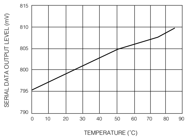
Fig. 10 Serial Data Output Level vs. Temperature
