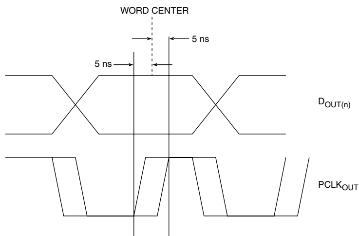
Fig. 21 Receiver Parallel Clock Alignment
