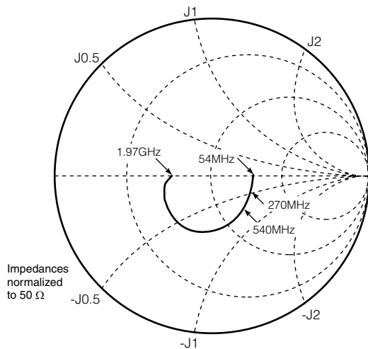
Fig. 16 Output Impedance
