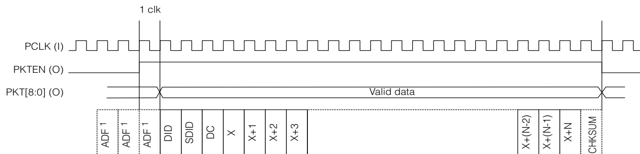
NOTE: 1 - The ancillary data flag, ADF, is one word in composite systems (ANSI/SMPTE 259M) and three words in component systems (ANSI/SMPTE 125M).
