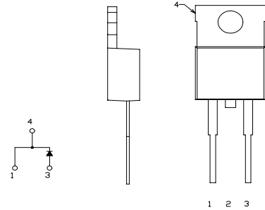
OUTLINE DRAWING
