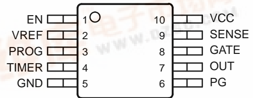
DGS Package (Top View)
