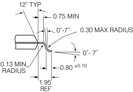
100 pin MQFP Dimensions in millimeters
