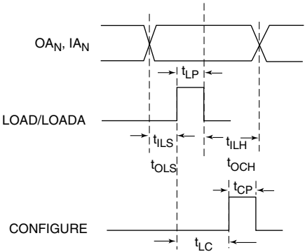
Fig. 6 LOAD/LOADA and Configure Timing
