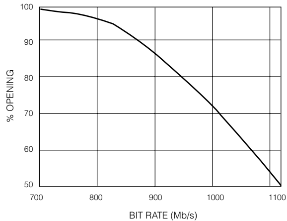
Fig. 2 Typical Eye Opening vs. Bit Rate
