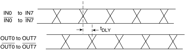
Fig. 5 GX9533 Data Latency
