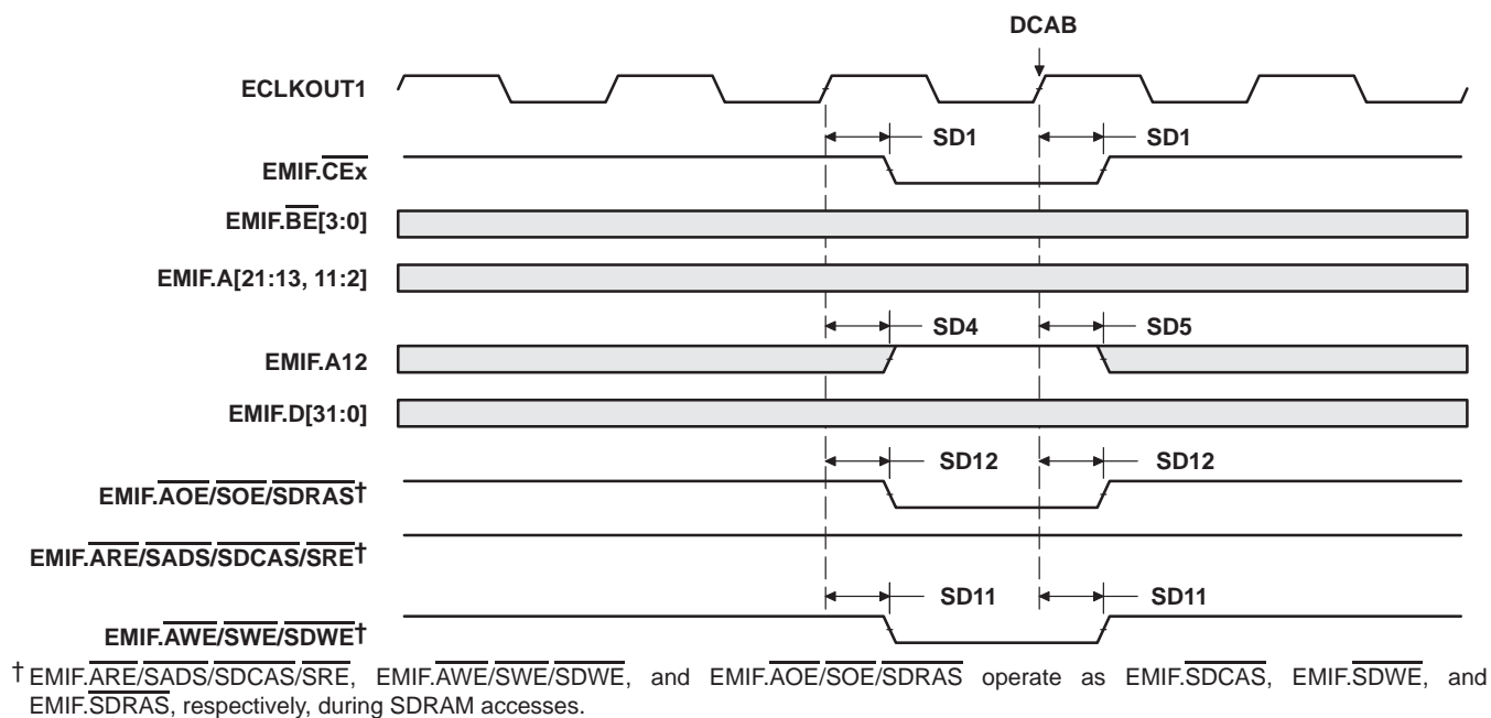
Figure 5–16. SDRAM DCAB Command
