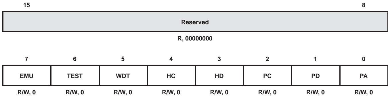
Figure 3-43. External Bus Control Register Layout (0x8800)
