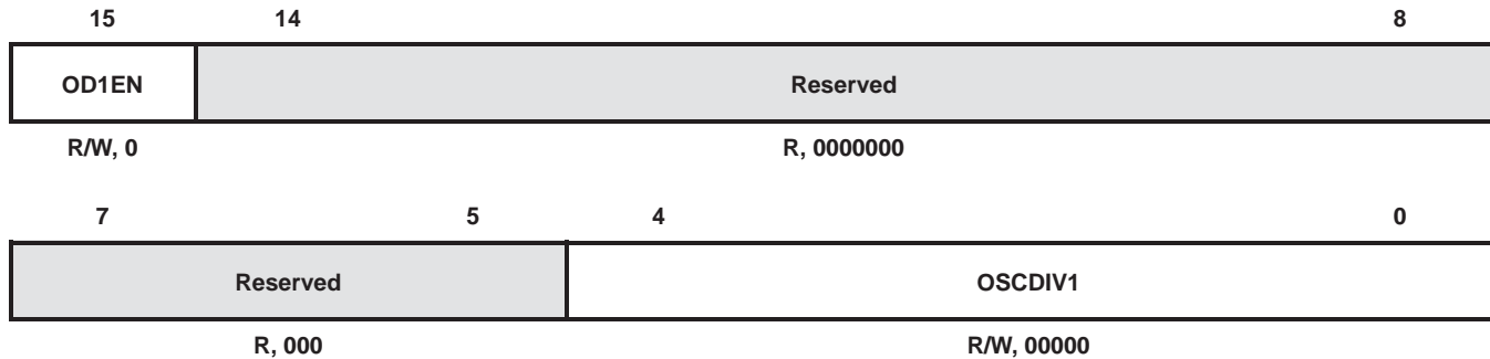
Figure 3–21. Oscillator Divider1 Register Layout (0x1C92)
