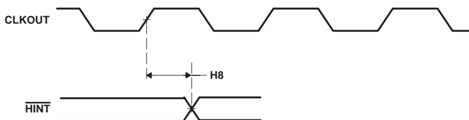
Figure 5–43. \overline{\text{HINT}} Timings
