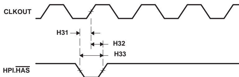
Figure 5–45. HPI. \overline{\text{HAS}} Interrupt Timings
