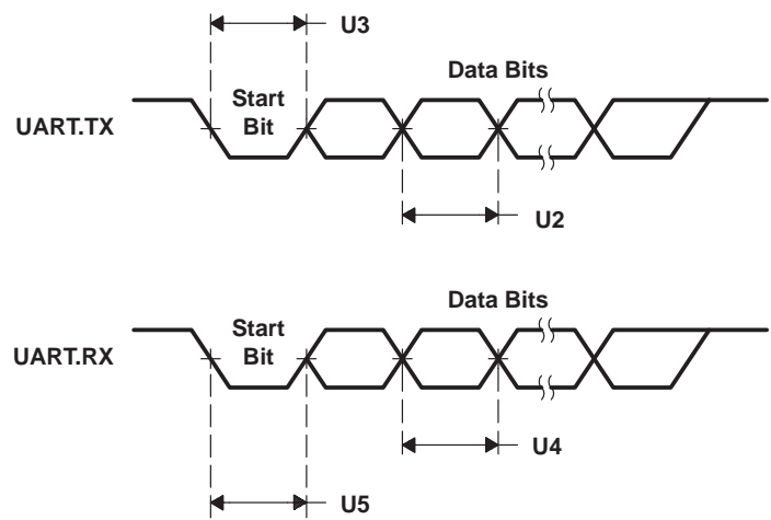
Figure 5–48. UART Timings
