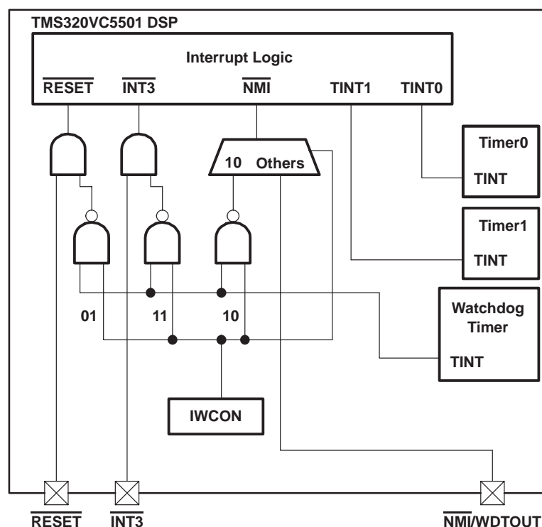
Figure 3–6. Timer Interrupts
