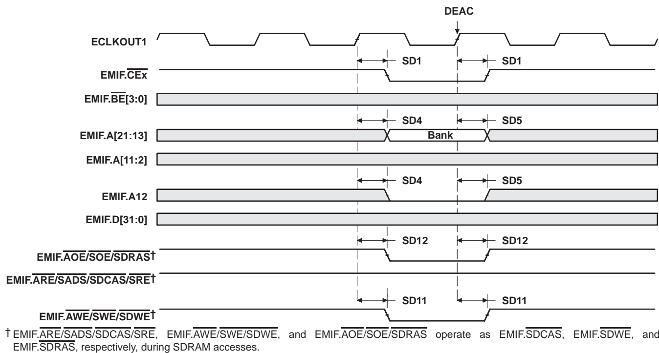
Figure 5–17. SDRAM DEAC Command
