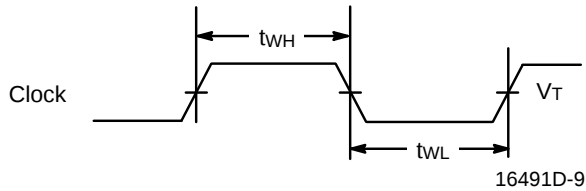
Clock Width
