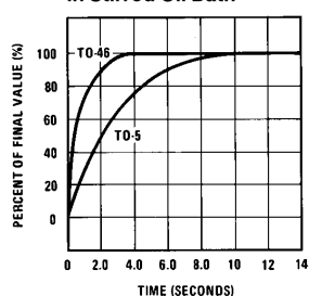
Thermal Time Constant in Stirred Oil Bath
