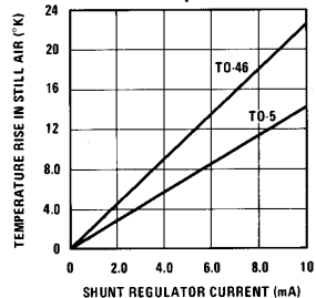
Device Temperature Rise
