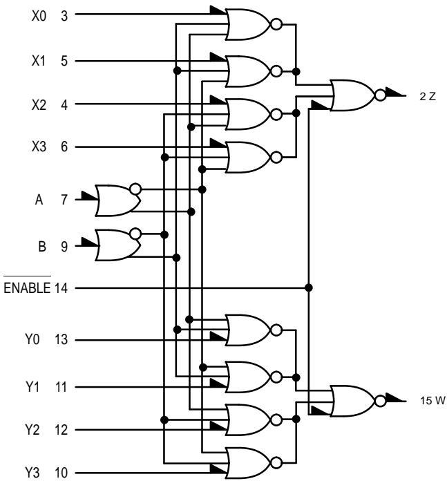
LOGIC DIAGRAM
