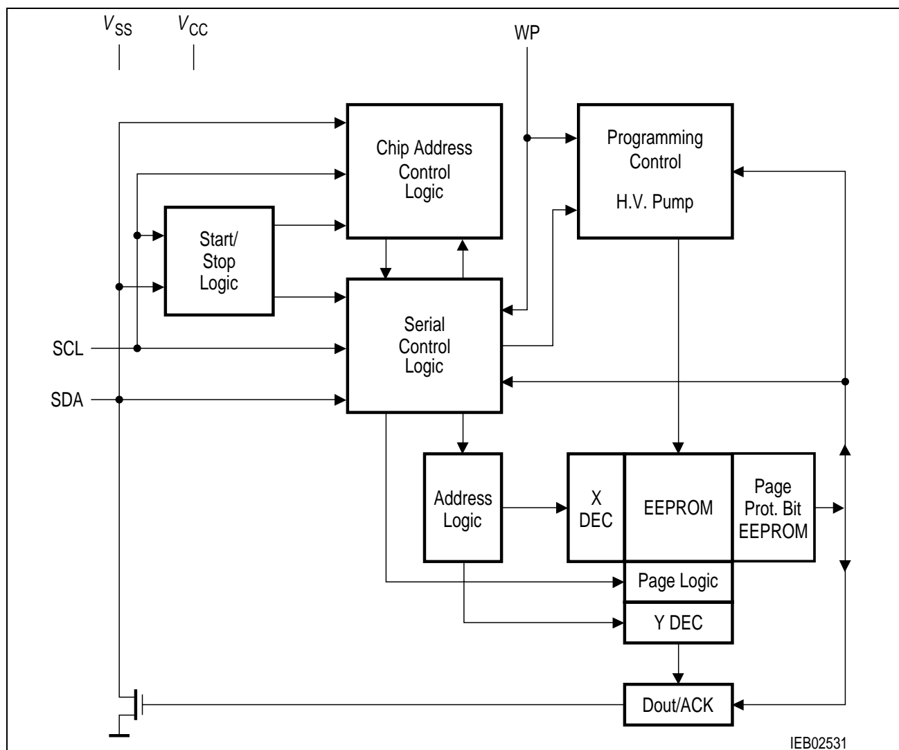
Figure 2 Block Diagram
