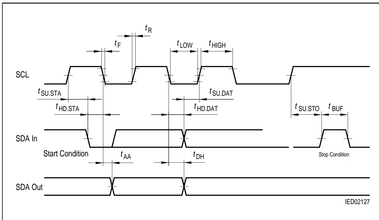
Figure 18 Bus Timing Data
