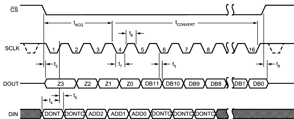
ADC78H89 Serial Timing Diagram
