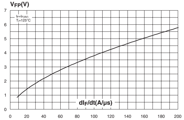
Figure 10: Transient peak forward voltage versus di_F/dt
