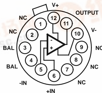
HA-2541/883 (METAL CAN) TOP VIEW
