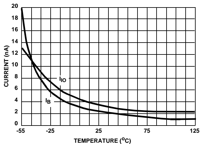
FIGURE 8. OFFSET CURRENT/BIAS CURRENT vs TEMPERATURE
