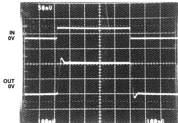
V_{OUT} = \pm 100mV , A_V = +5 , R_L = 1K , C_L \leq 10pF
