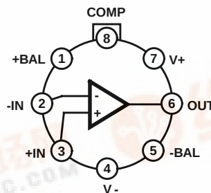
HA-2548/883 (METAL CAN) TOP VIEW
