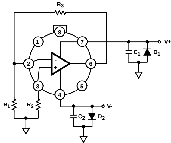
HA2-2548/883 METAL CAN
