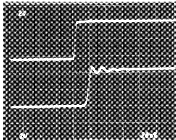
DRIVING HA5023 AS I TO V CONVERTER V_X FULLPOWER BANDWIDTH
