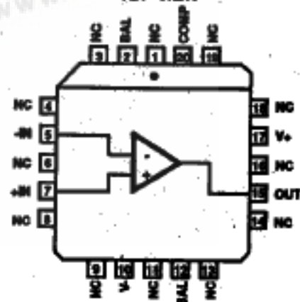
HA-2625, (PLCC) TOP VIEW
