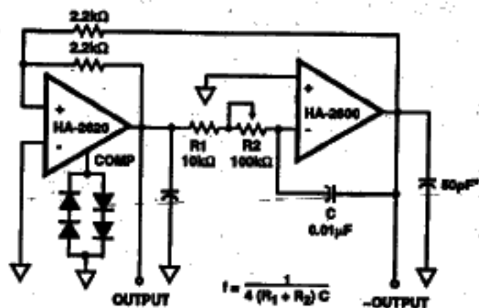
FIGURE 11. FUNCTION GENERATOR
