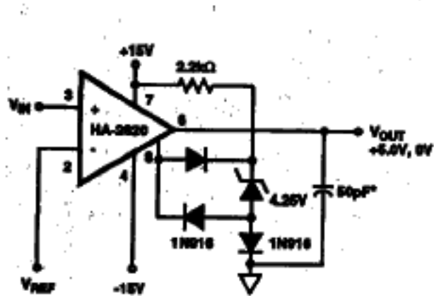
FIGURE 10. HIGH IMPEDANCE COMPARATOR
