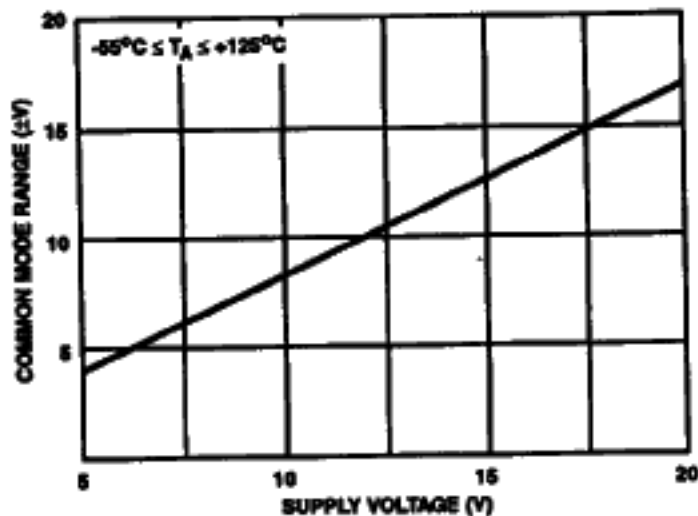
FIGURE 7. COMMON MODE VOLTAGE RANGE vs SUPPLY VOLTAGE
