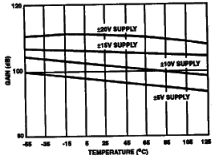
FIGURE 8. OPEN LOOP VOLTAGE GAIN vs TEMPERATURE
