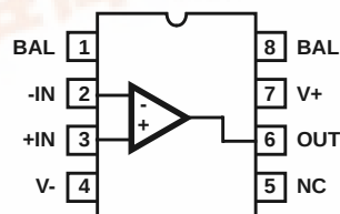
HA-2841/883 (CERDIP) TOP VIEW
