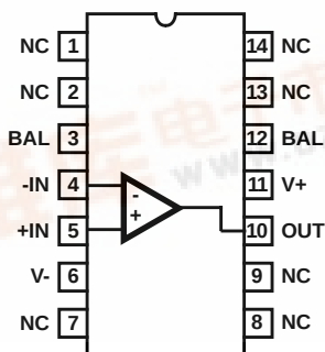
HA-2841/883 (CERDIP) TOP VIEW
