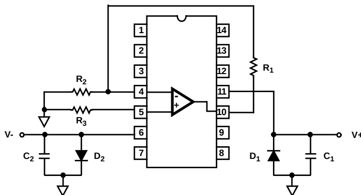
HA1-2841/883 CERAMIC DIP
