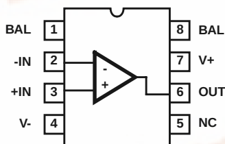
HA-5137A (CERDIP) TOP VIEW
