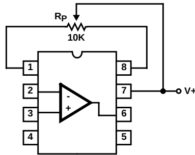
FIGURE 3. SUGGESTED OFFSET VOLTAGE ADJUSTMENT
