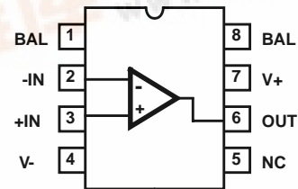
HA-5147 (CERDIP, SOIC) TOP VIEW
