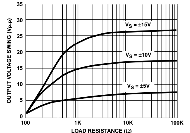
FIGURE 15. MAXIMUM OUTPUT VOLTAGE SWING vs LOAD RESISTANCE
