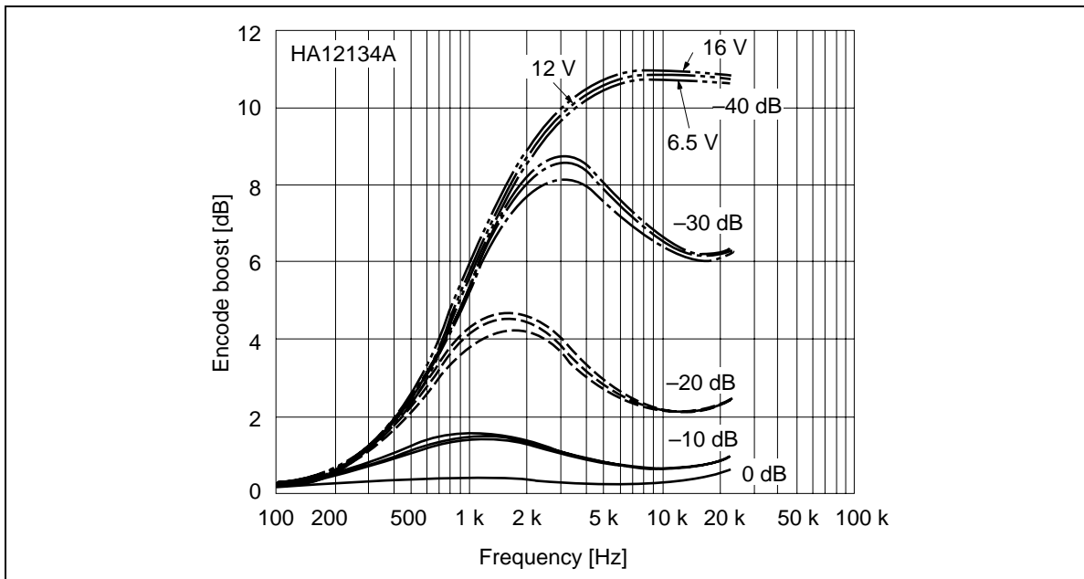
Figure 26 Encode Boost vs. Frequency
