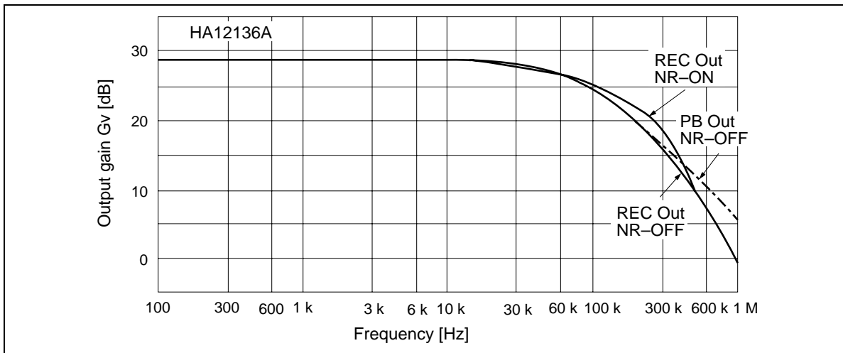
Figure 6 PB Mode Output Gain vs. Frequency
