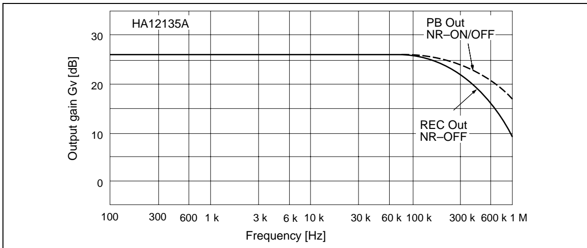
Figure 16 REC Mode Output Gain vs. Frequency
