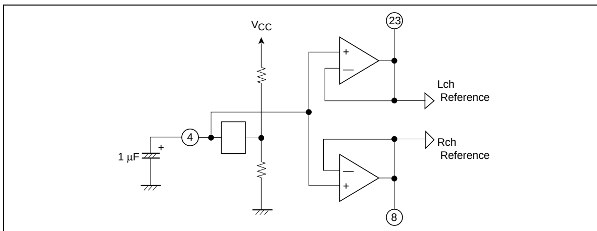
Figure 1 The Block-Diagram of Reference Voltage Supply
