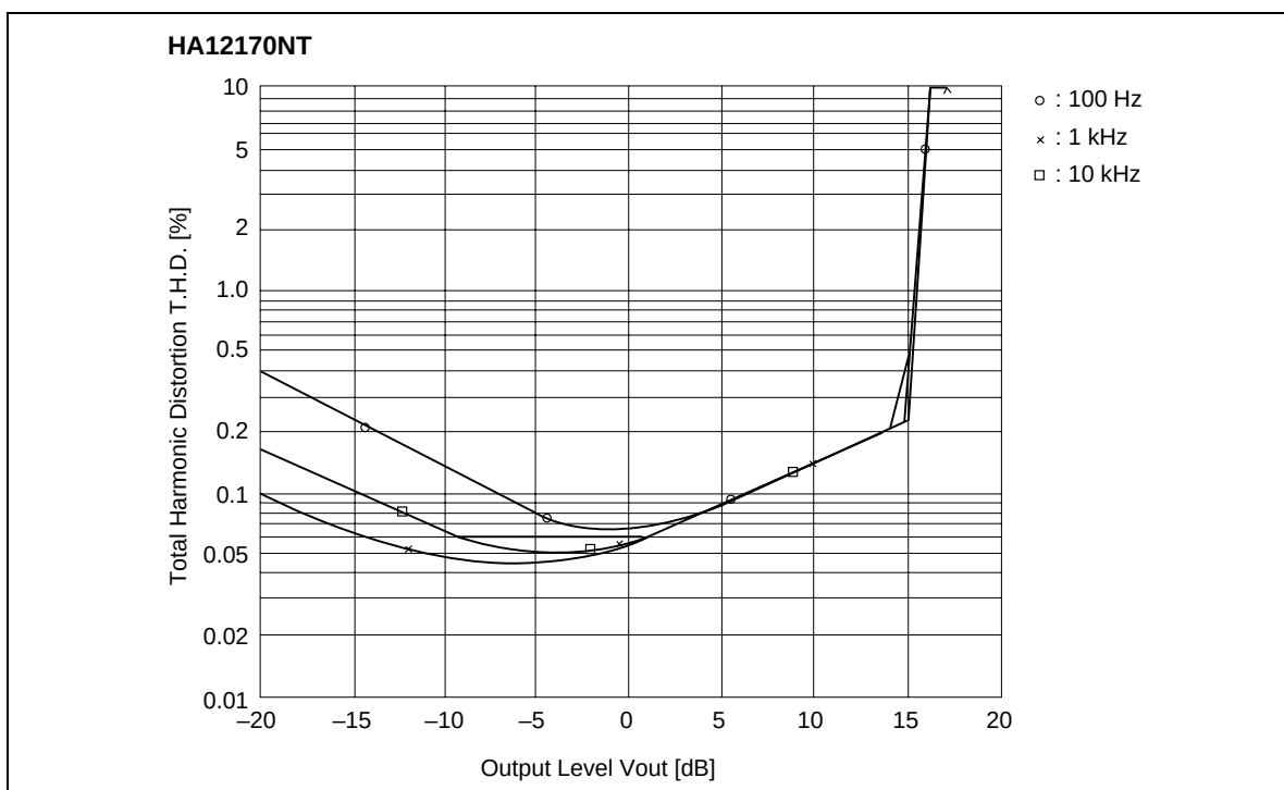
Total Harmonic Distortion vs. Output Level (PB MODE NR-B V_{CC} = 14 V)
