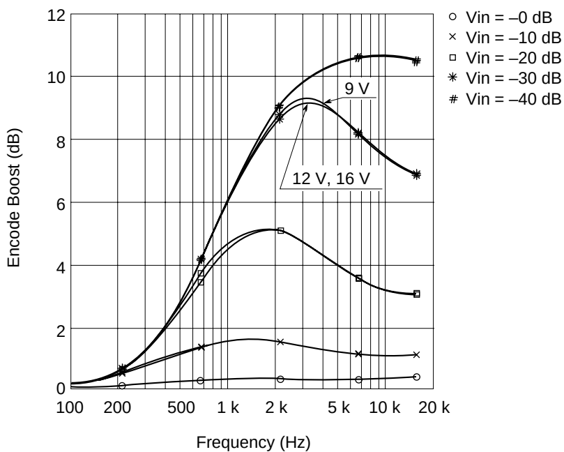
Encode Boost vs. Frequency (NR-B, V_{CC} = 9 \text{ V}, 12 \text{ V}, 16 \text{ V} )
