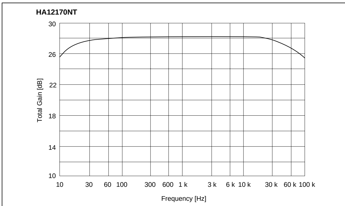
Total Gain vs. Frequency (PB MODE PBOUT NR-OFF V_{CC} = 14\text{ V} )
