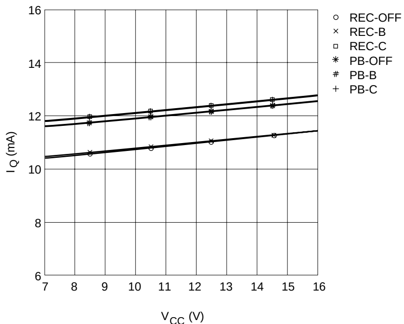
Quiescent Circuit vs. Supply Voltage
