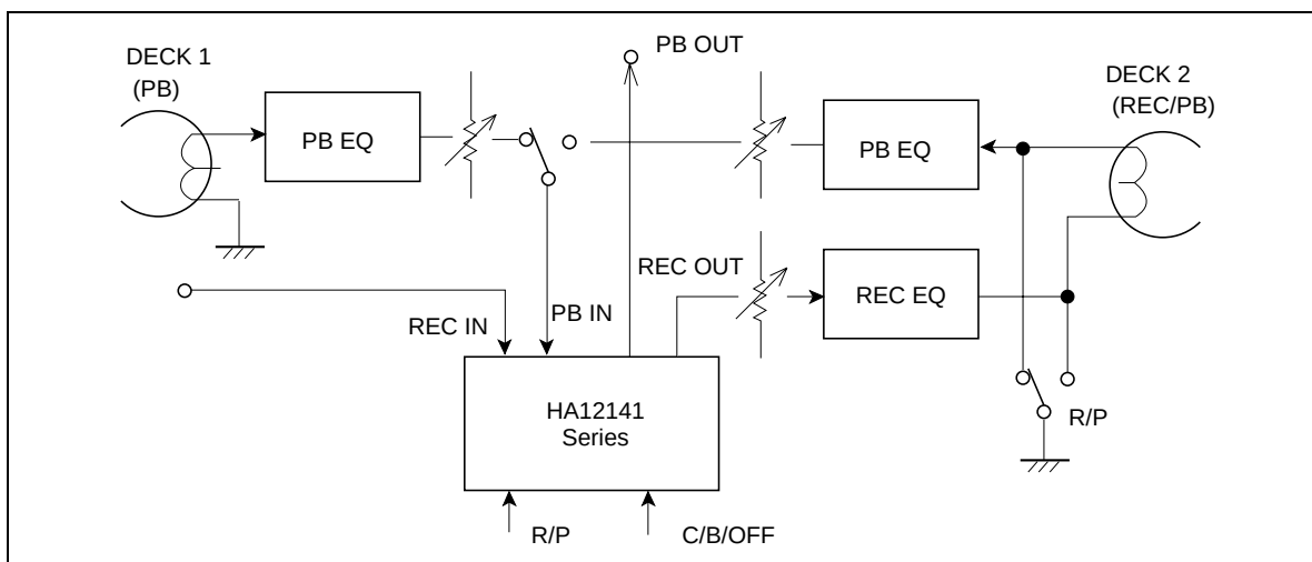
Figure 5 Application for Dubbing Deck
