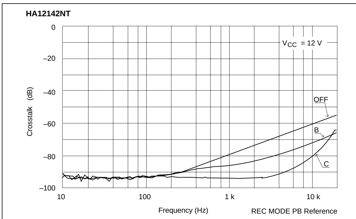
Crosstalk vs. Frequency (REC→PB)
