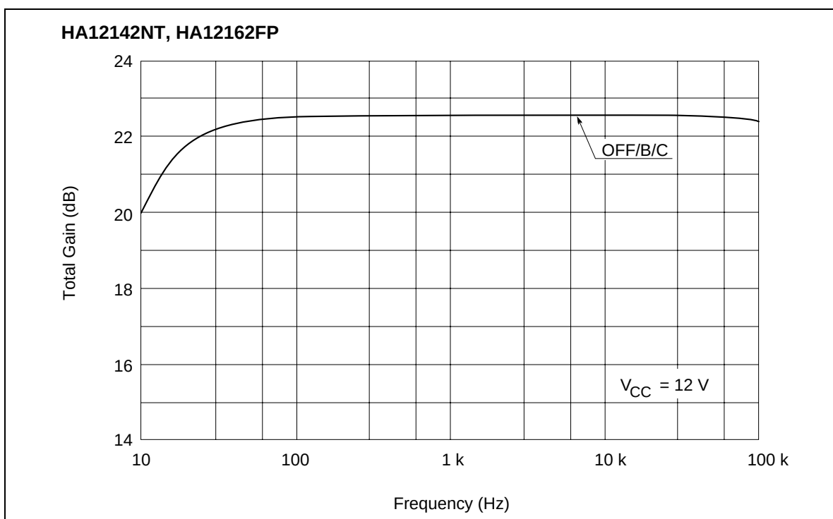
Total Gain vs. Frequency (REC MODE PBOUT)
