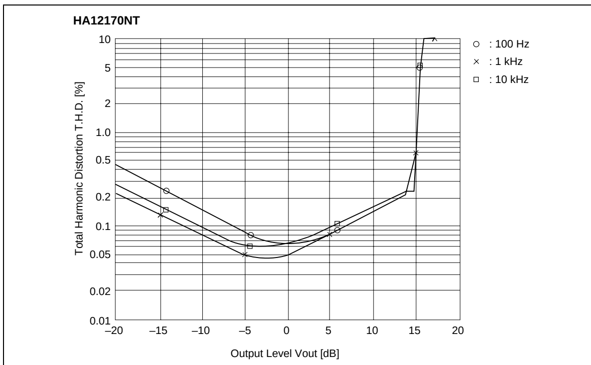
Total Harmonic Distortion vs. Output Level (PB MODE NR-OFF V_{CC} = 14 V)
