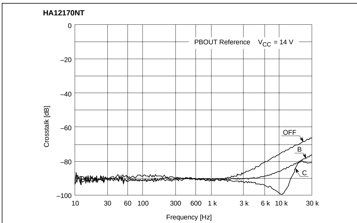
Crosstalk vs. Frequency (PB MODE R↔L)
