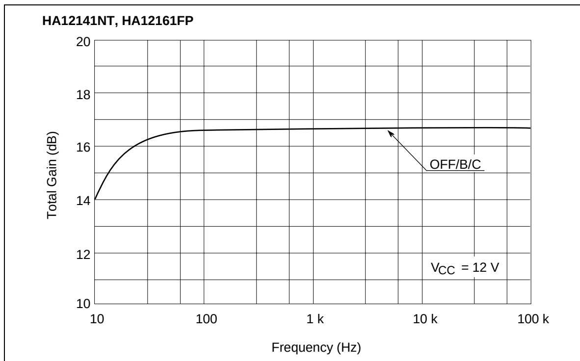
Total Gain vs. Frequency (REC MODE PBOU)
