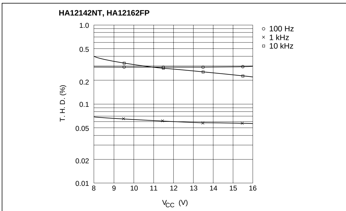
Total Harmonic Distortion vs. Supply Voltage (PB MODE NR-C)
