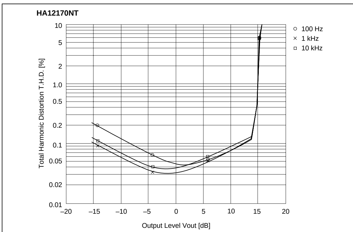
Total Harmonic Distortion vs. Output Level (REC MODE NR-OFF V_{CC} = 14\text{ V} )
