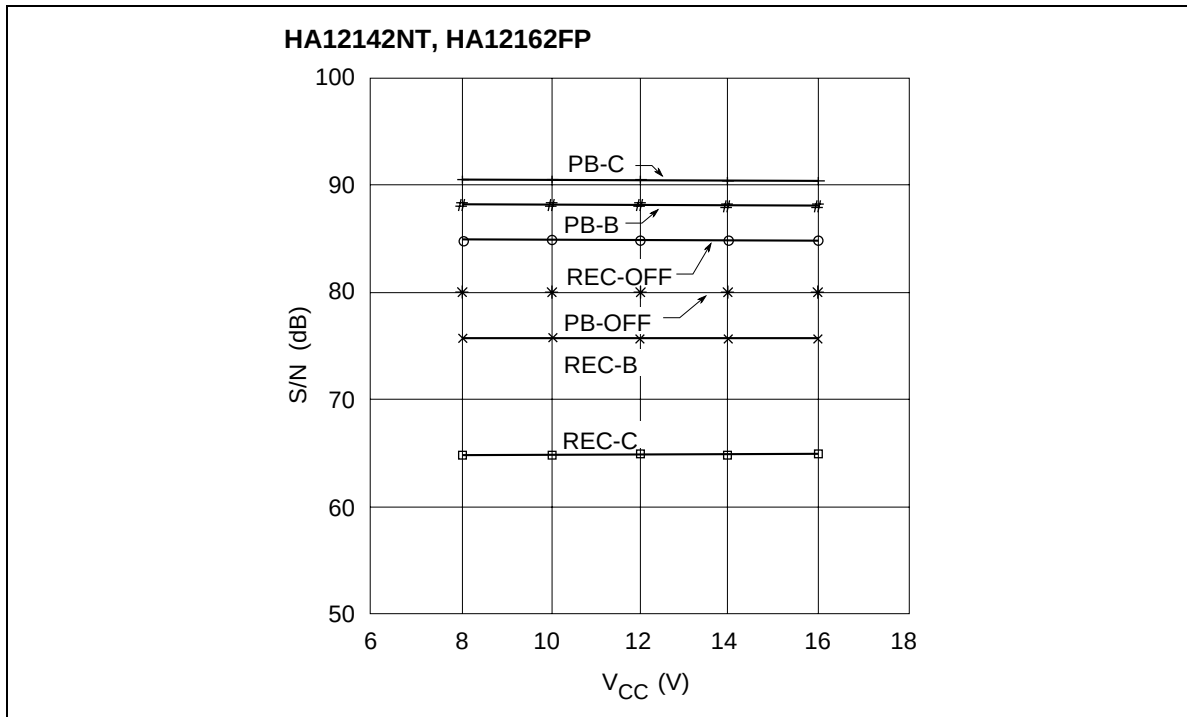
S/N vs. Supply Voltage
