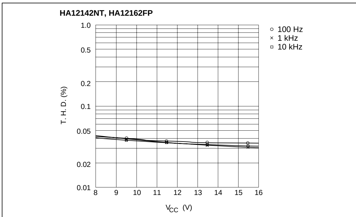
Total Harmonic Distortion vs. Supply Voltage (PB MODE NR-B)
