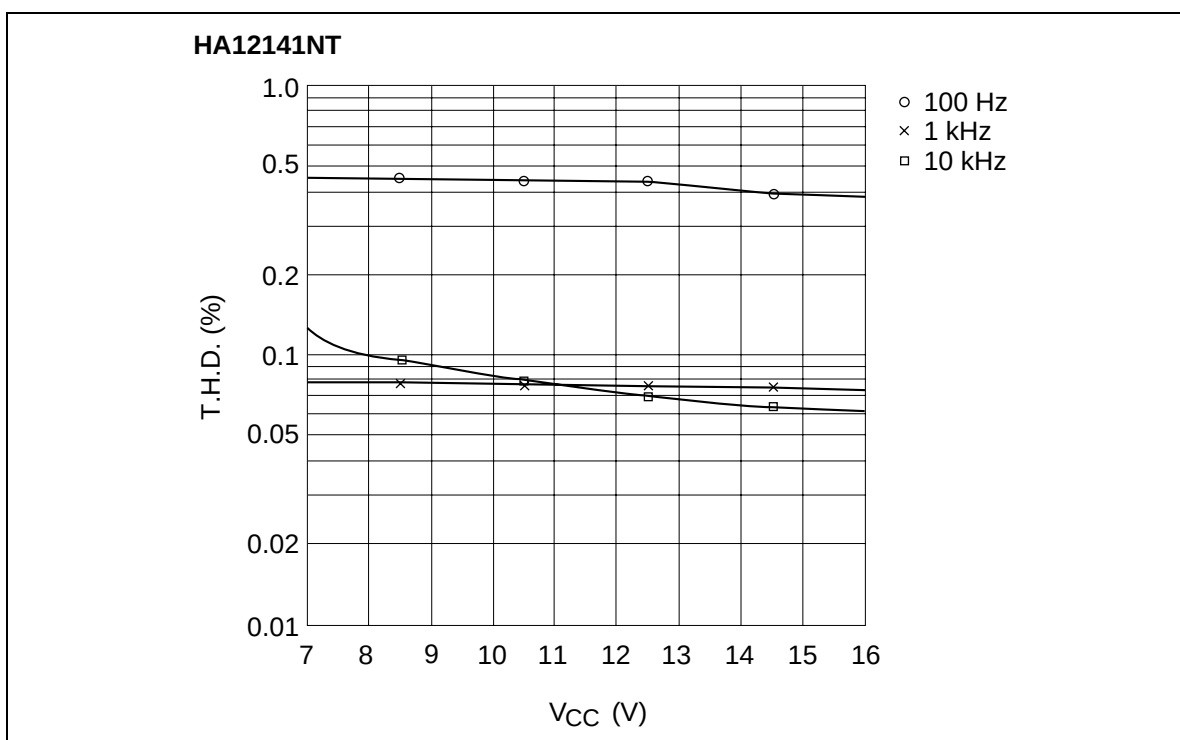
Total Harmonic Distortion vs. Supply Voltage (REC MODE NR-C)
