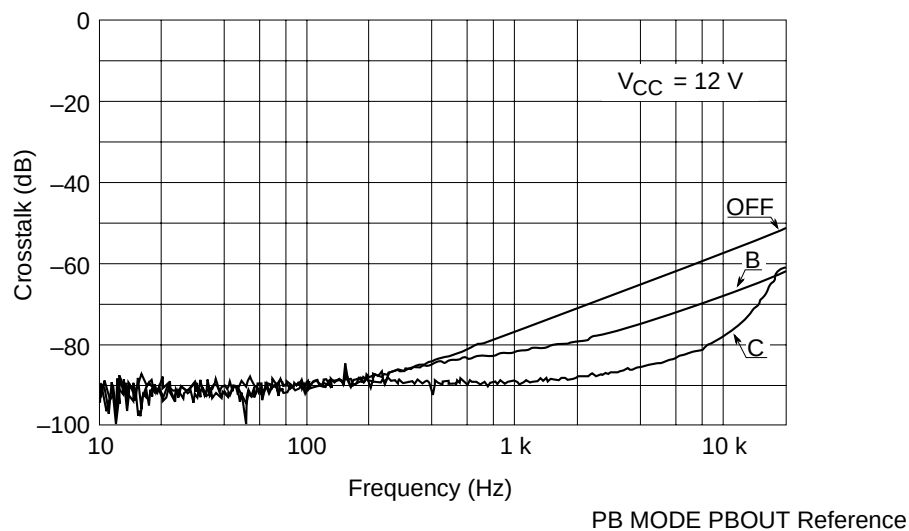
Crosstalk vs. Frequency (REC→PB)
