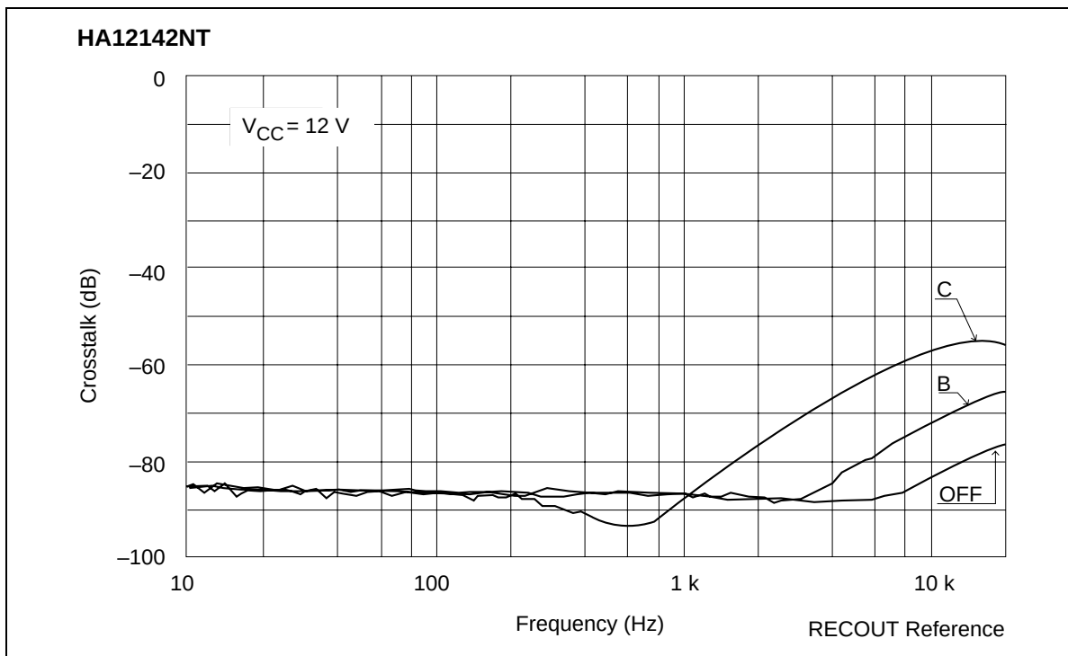
Crosstalk vs. Frequency (REC MODE R↔L)
