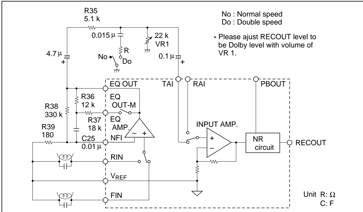
Figure 7 Application Circuit for Double Speed
