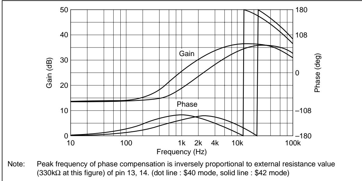
Figure 16 Tracking Servo Frequency Characteristic (pin 11, 12 are open)
