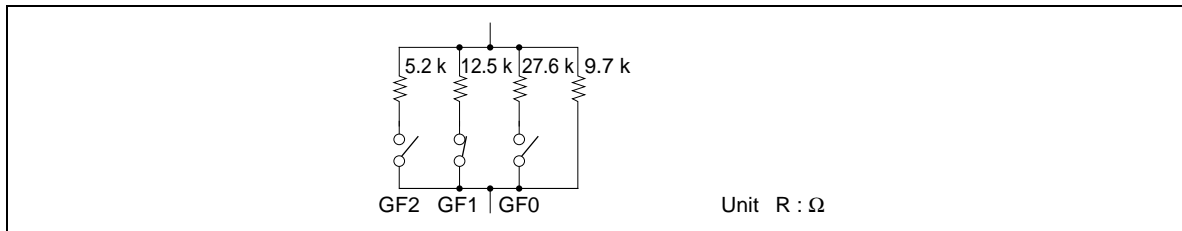
Figure 4 Focus VR
