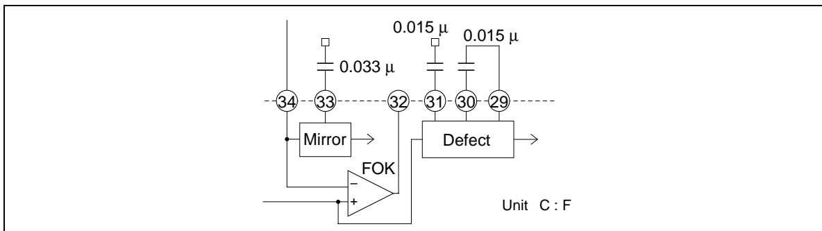
Figure 8 Mirror, FOK, and Defect Detectors
