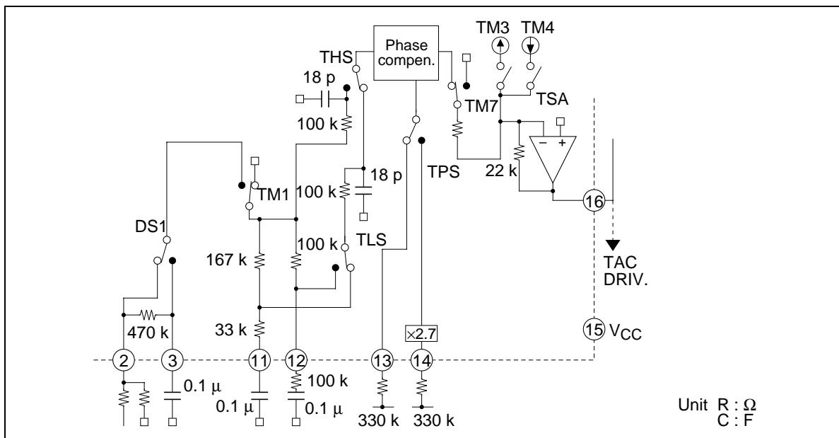
Figure 15 Tracking Servo
