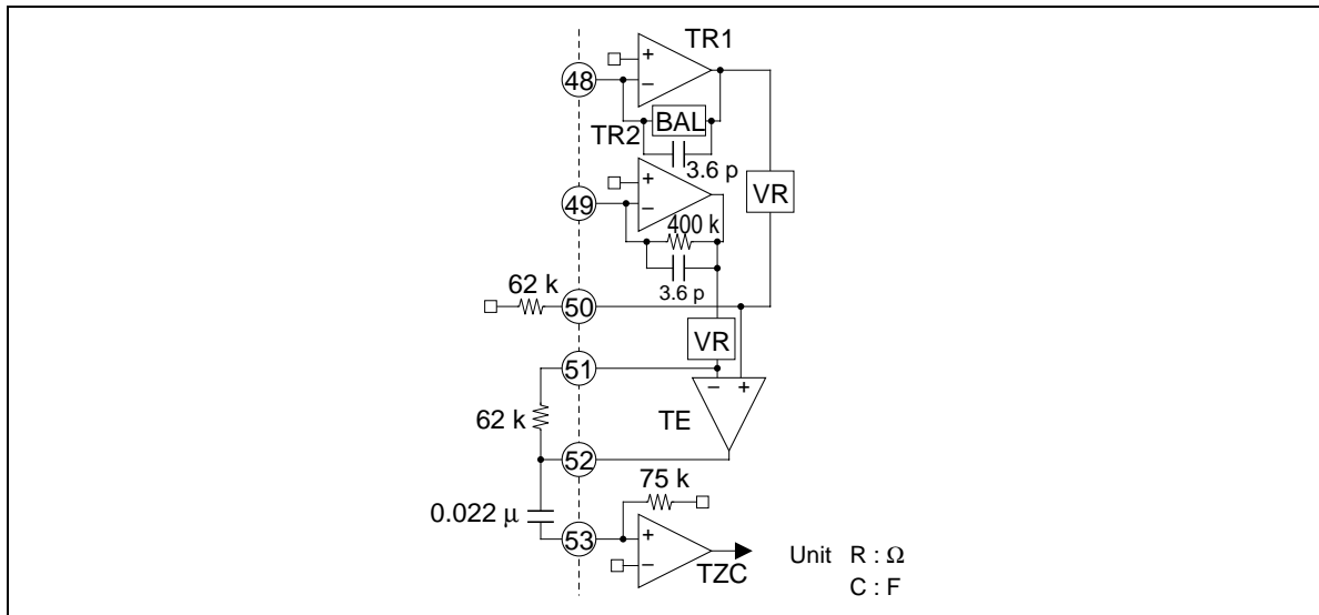
Figure 5 Tracking Pre-Amplifiers
