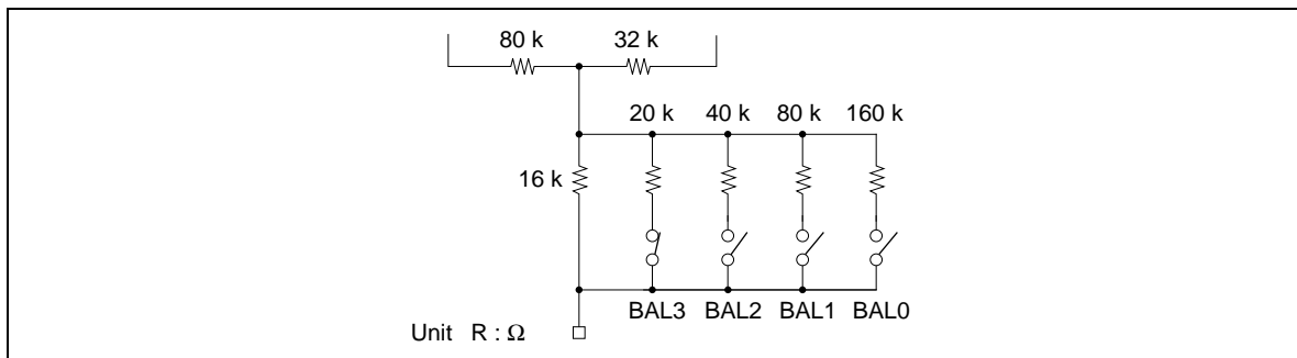
Figure 6 BAL
