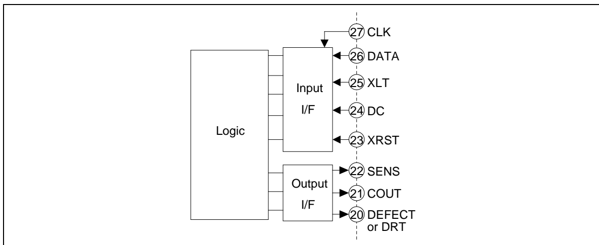
Figure 2 Microprocessor Interface
