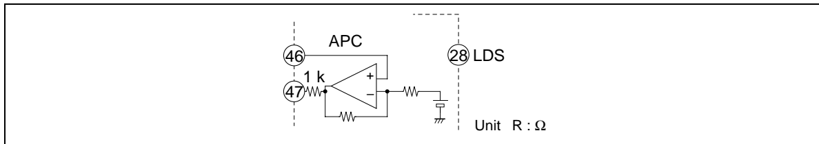
Figure 12 APC
