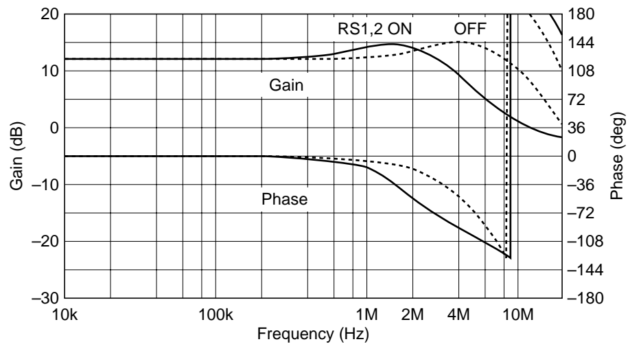
Figure 3-A Frequency characteristic example of RF preamplifiers
