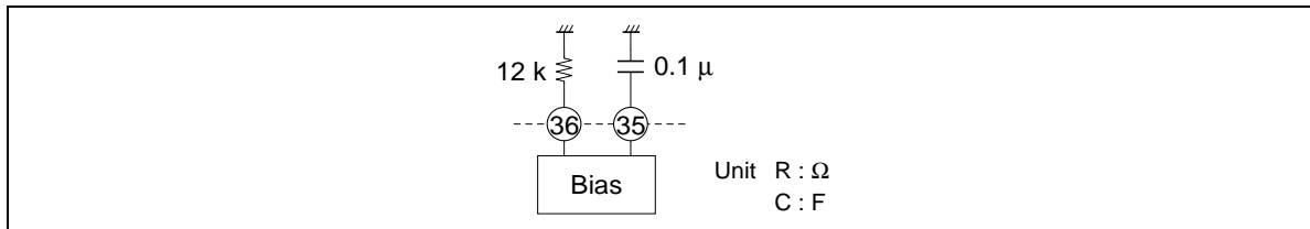
Figure 11 Bias
