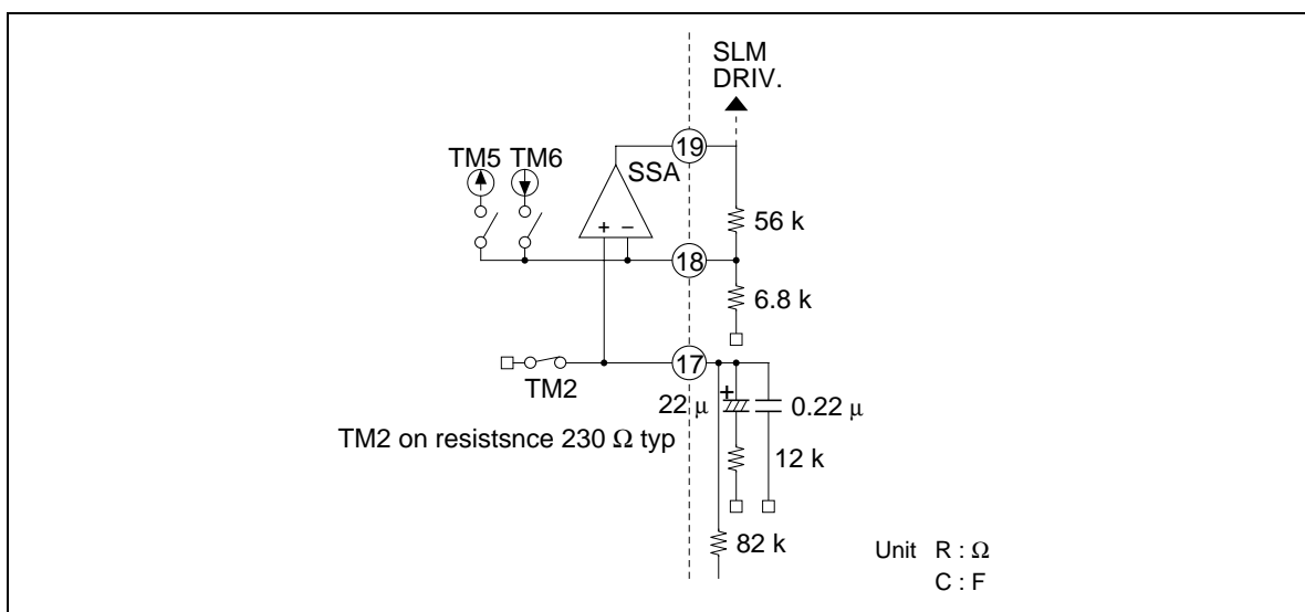
Figure 19 Sled Servo
