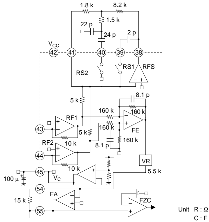
Figure 3 RF and Focus Error Pre-Amplifiers
