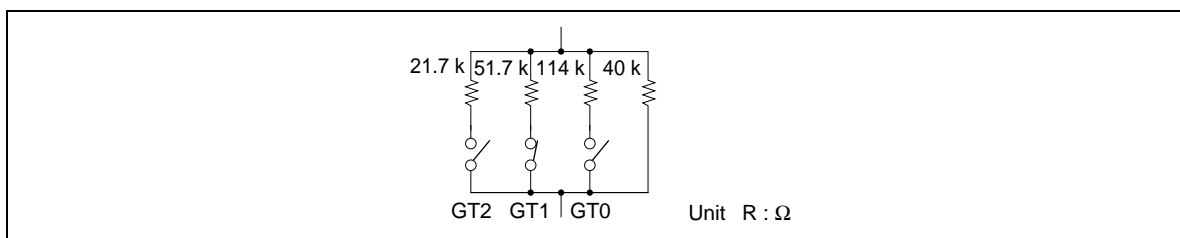
Figure 7 Tracking VR
