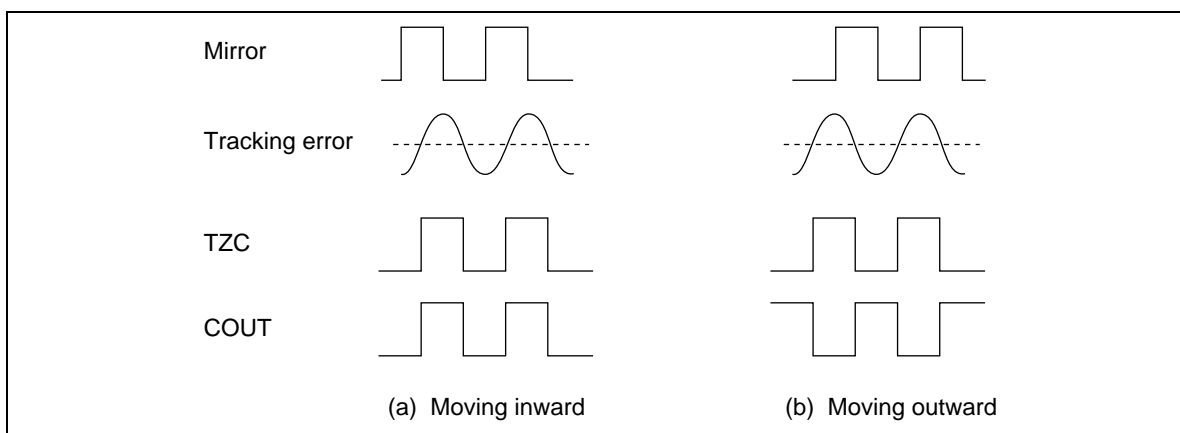
Figure 17 Phase Relationships of Mirror and Other Signals
