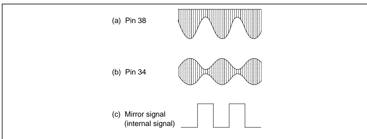
Figure 10 Mirror Detector Waveforms
