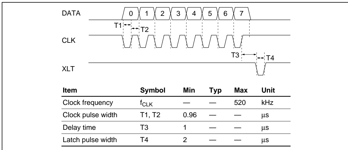
Figure 1 Timing Diagram for Microprocessor Control
