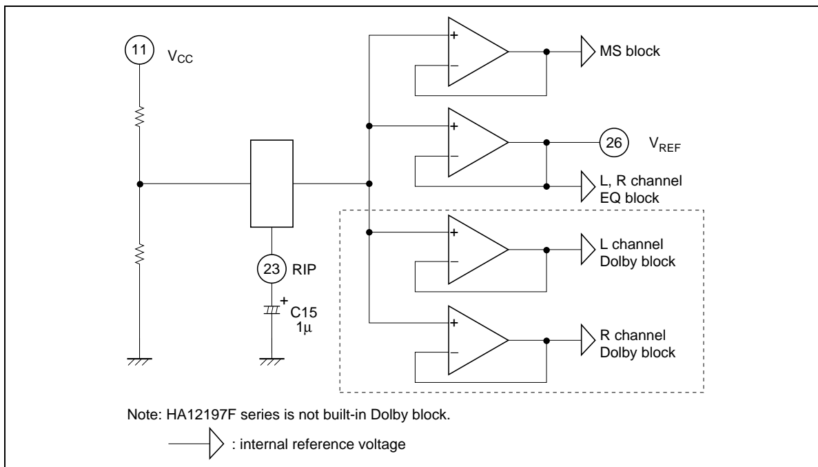
Figure 1 The Block Diagram of Reference Supply Voltage
