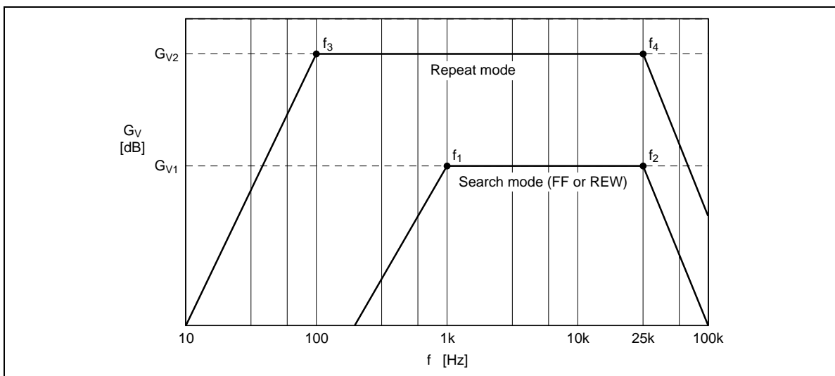
Figure 5 Frequency Response
