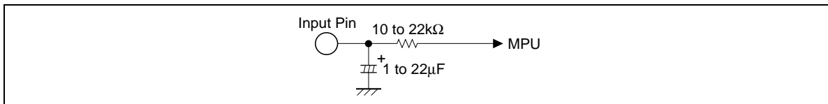
Figure 2 Interface for Reduction of Pop Noise
