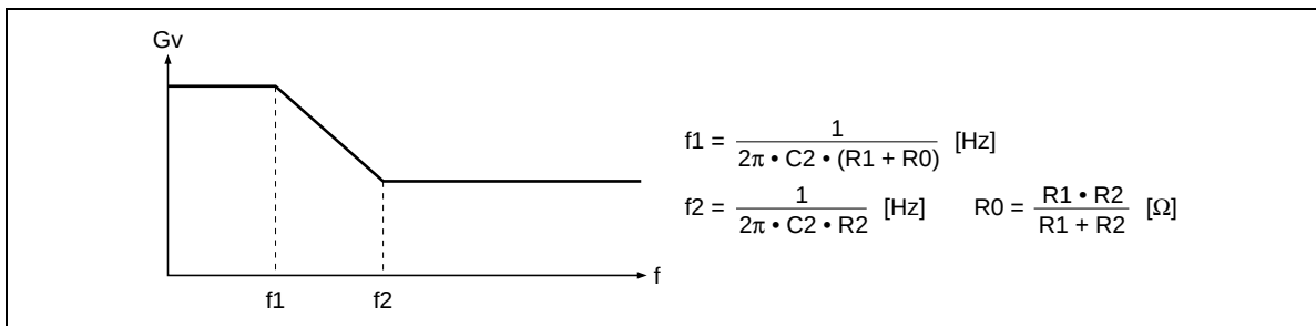
Figure 9 Frequency Characteristic of Low-Boost
