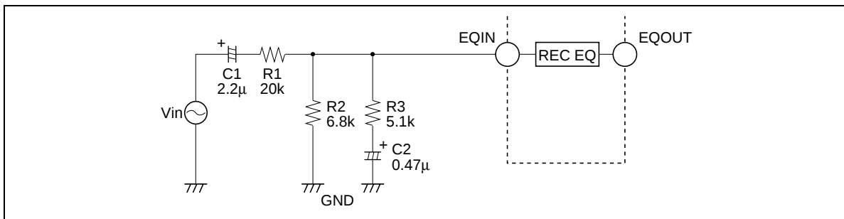
Figure 8 Example of Low Boost Circuit
