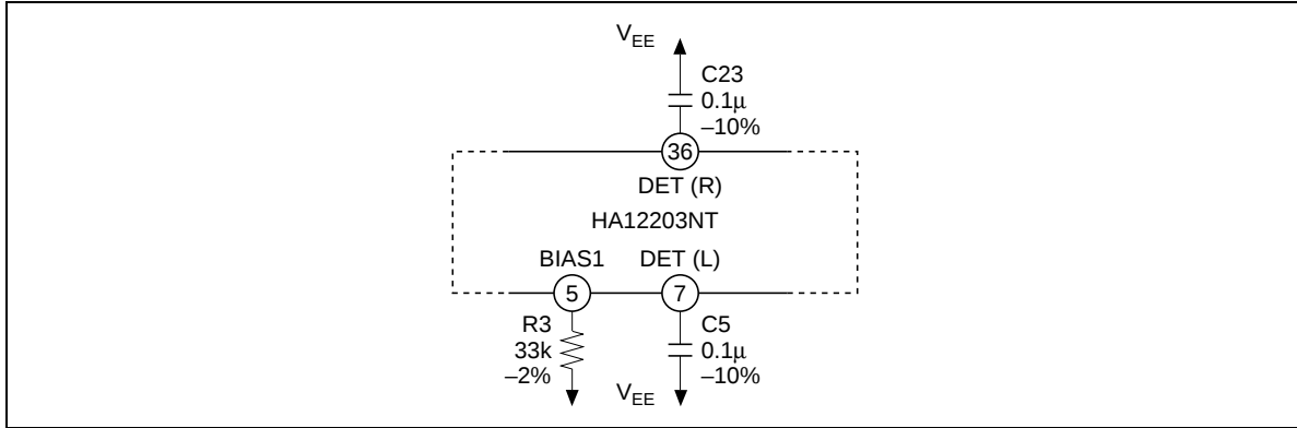
Figure 7 Tolerance of External Components
