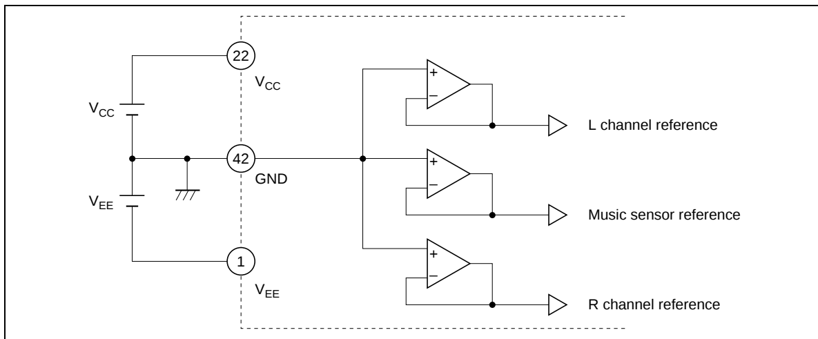
Figure 1 Reference Voltage
