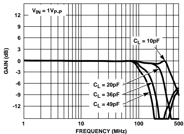
FIGURE 5. FREQUENCY RESPONSE
