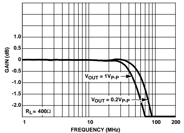
FIGURE 16. GAIN FLATNESS
