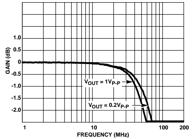
FIGURE 14. GAIN FLATNESS
