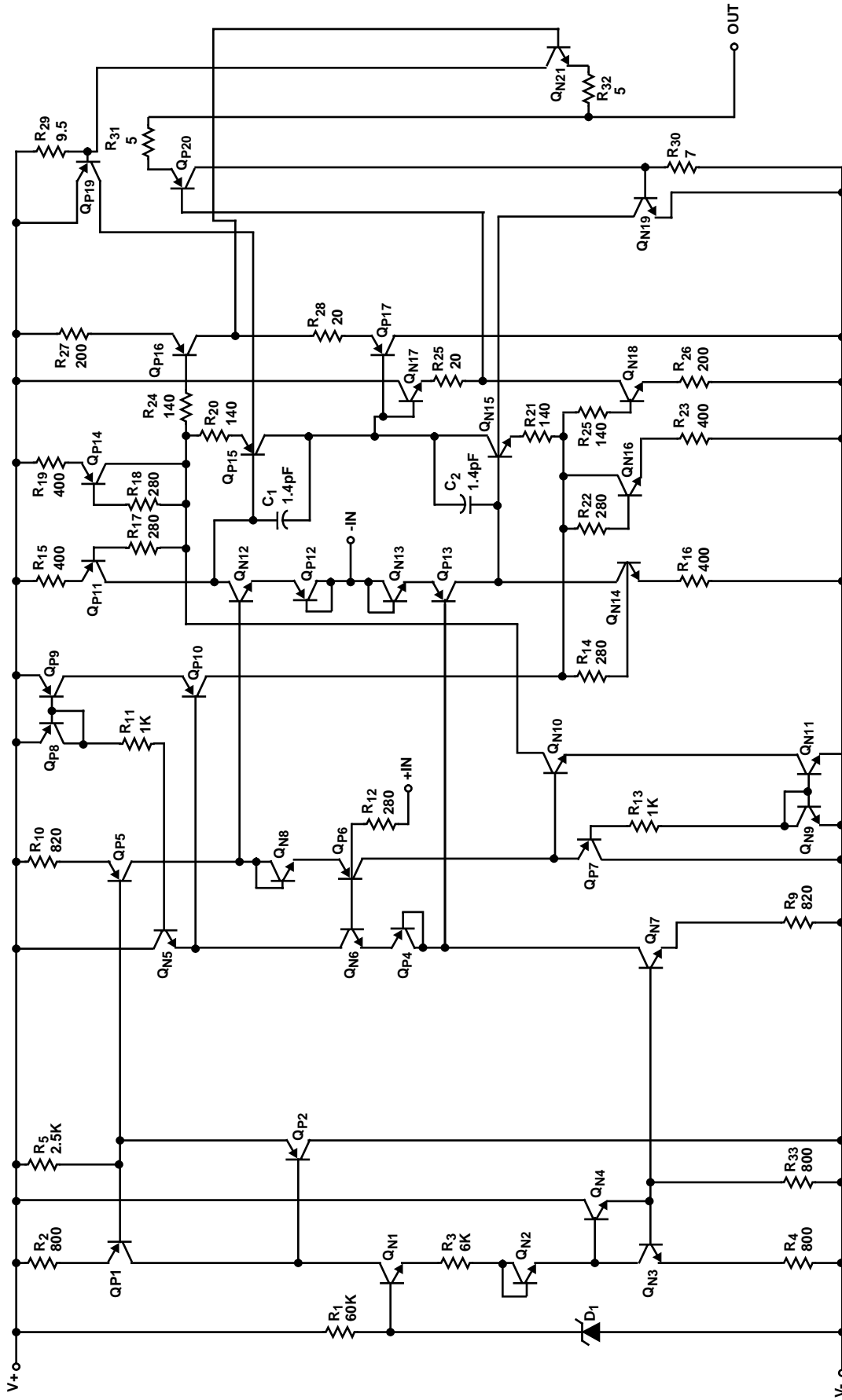
Schematic (One Amplifier of Three)
