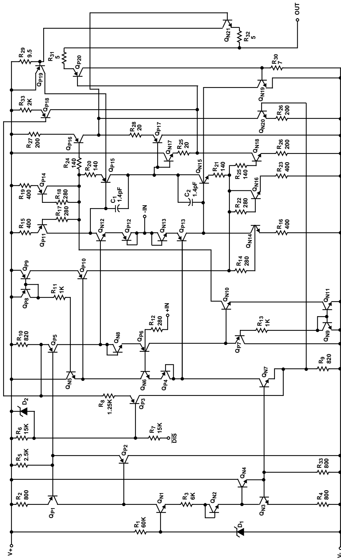
Schematic Diagram (One Amplifier of Two)
