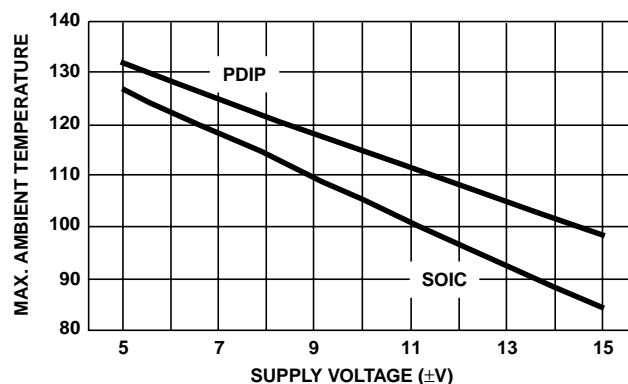
FIGURE 7. MAXIMUM OPERATING AMBIENT TEMPERATURE vs SUPPLY VOLTAGE
