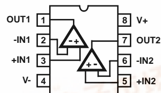
HA5023 (PDIP, SOIC) TOP VIEW
