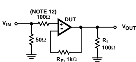
FIGURE 2. SMALL SIGNAL PULSE RESPONSE CIRCUIT
