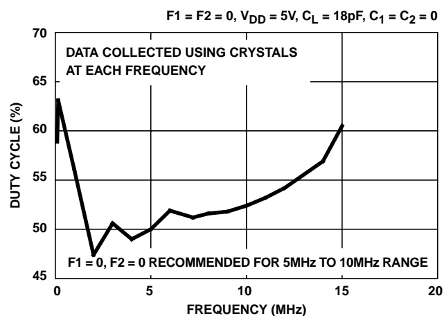
FIGURE 25. DUTY CYCLE vs FREQUENCY
