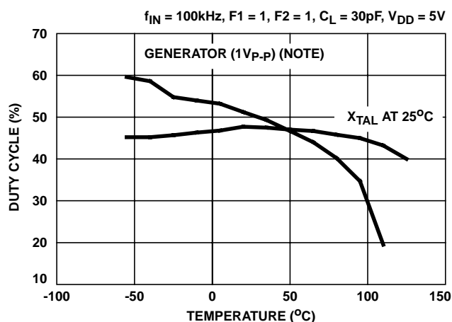
FIGURE 24. DUTY CYCLE vs TEMPERATURE
