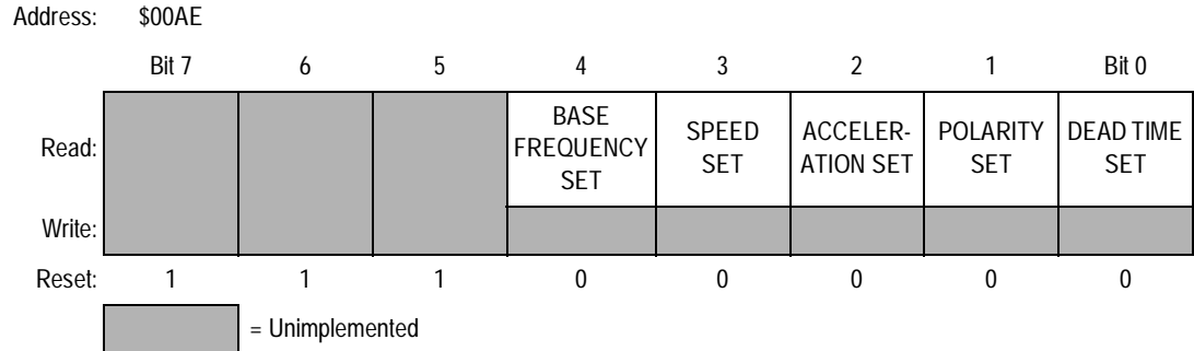
Figure 15. Setup Register
