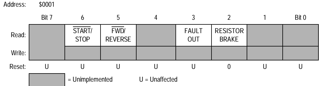
Figure 16. Switch In Register
