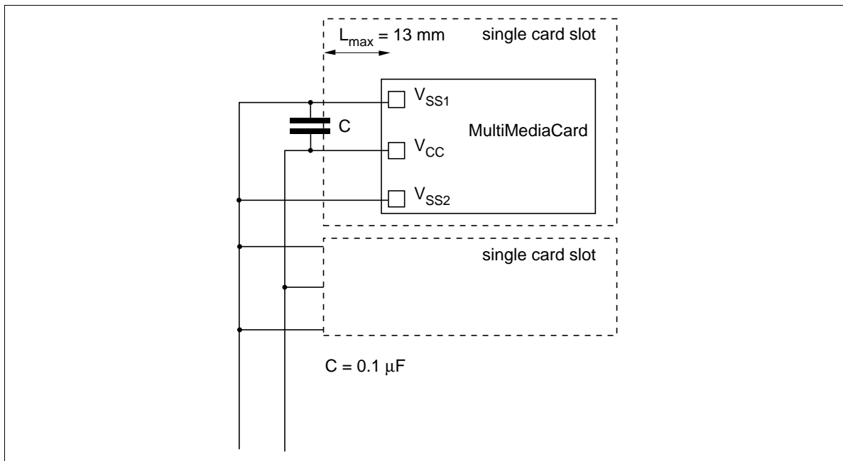
Power Supply Decoupling
