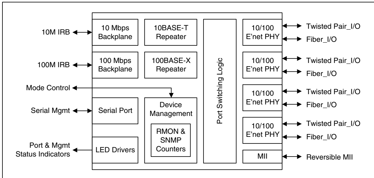
Figure 1. LXT980/980A Dual-Speed, 5-Port Fast Ethernet Repeater
