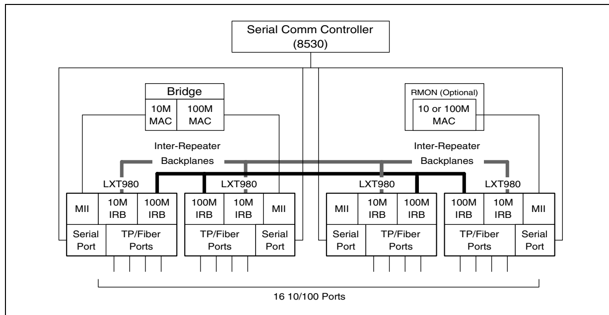
Figure 16. Hybrid Switch/Repeater Application - for Balanced 10/100 Performance
