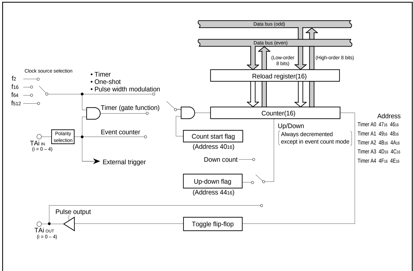
Fig. 13 Block diagram of timer A
