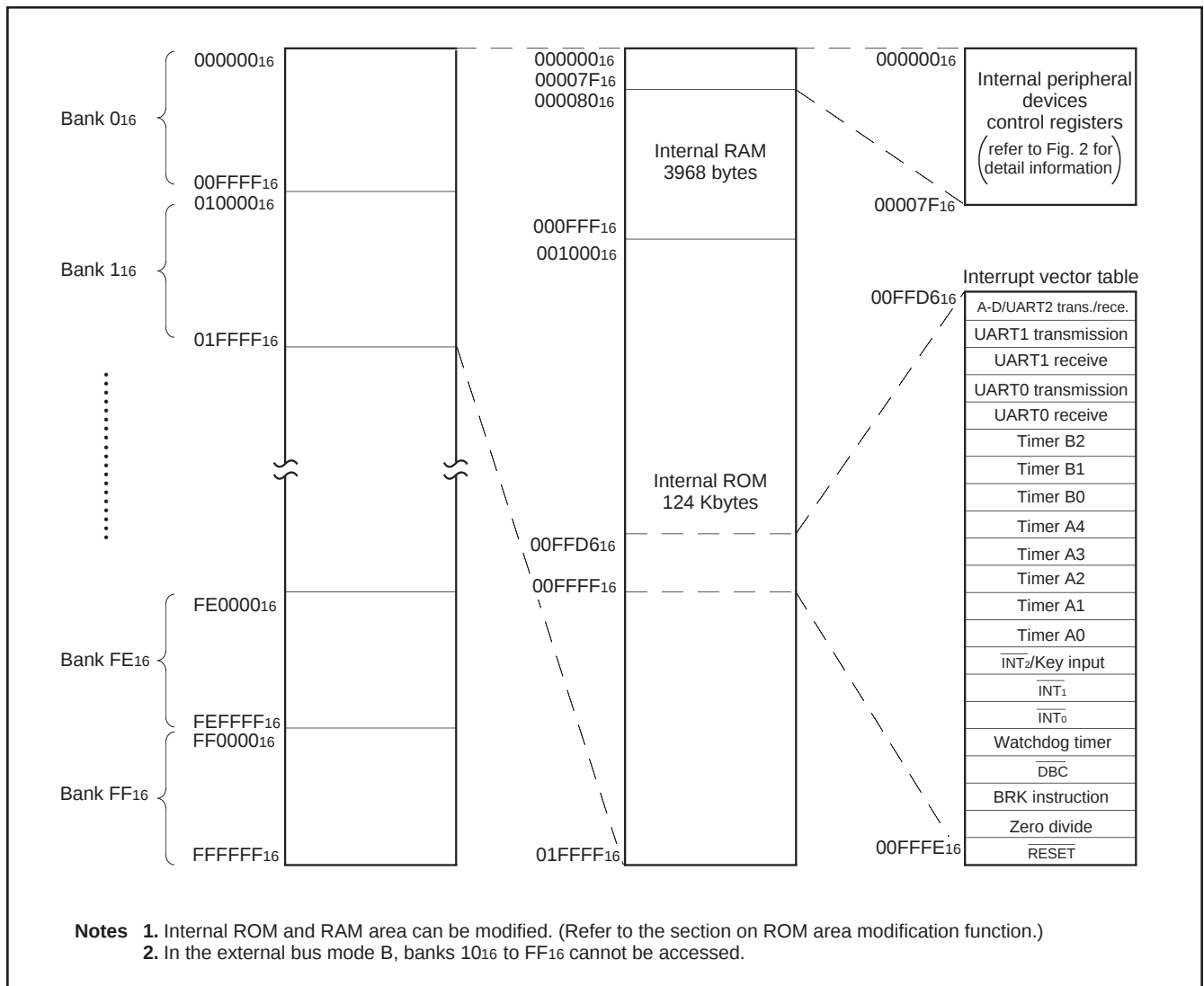
Fig. 1 Memory map
