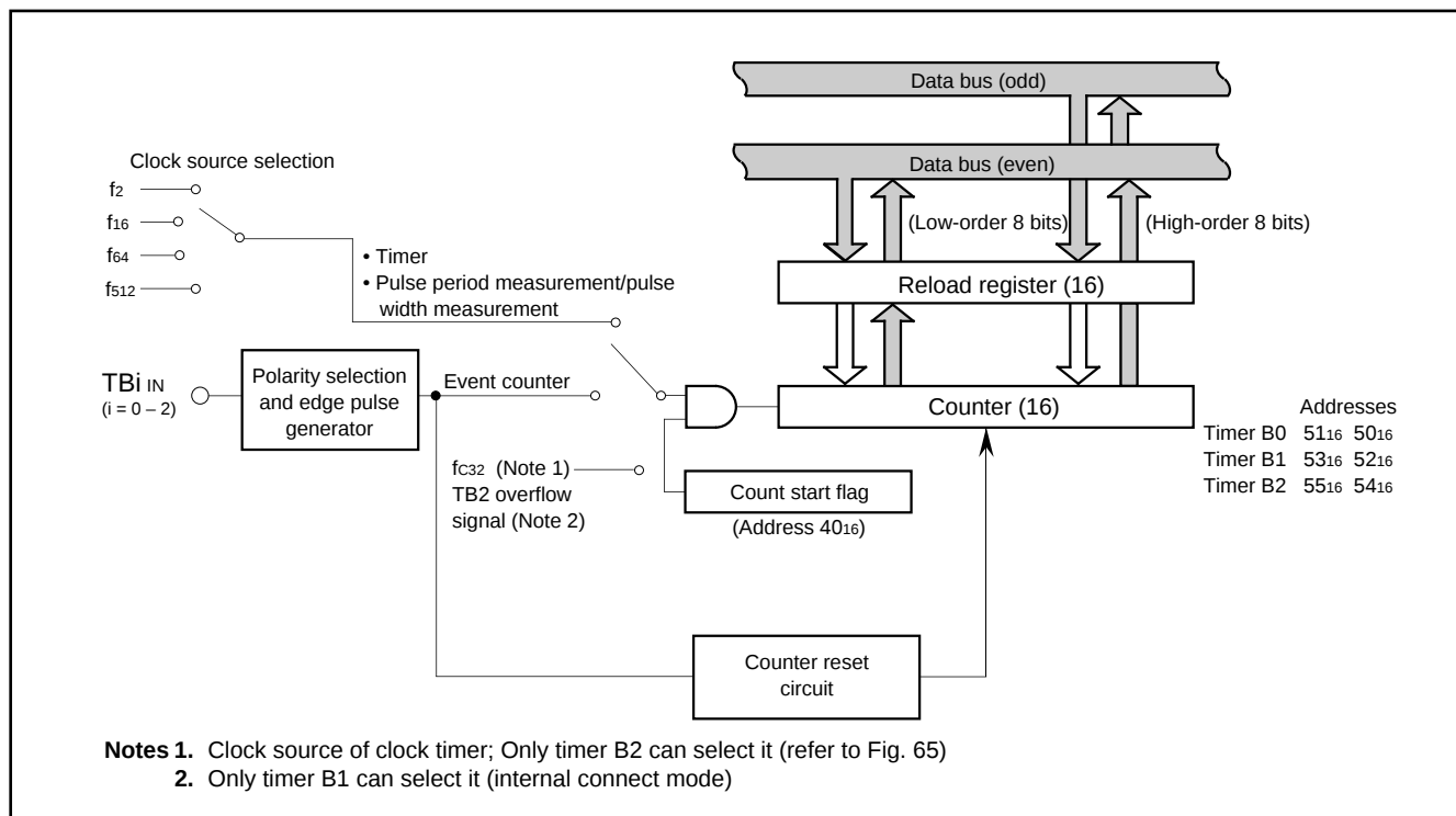
Fig. 29 Timer B block diagram
