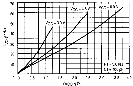
Figure 12B. VCO Frequency ( f_{VCO} ) as a Function of the VCO Input Voltage ( V_{VCO\_IN} )
