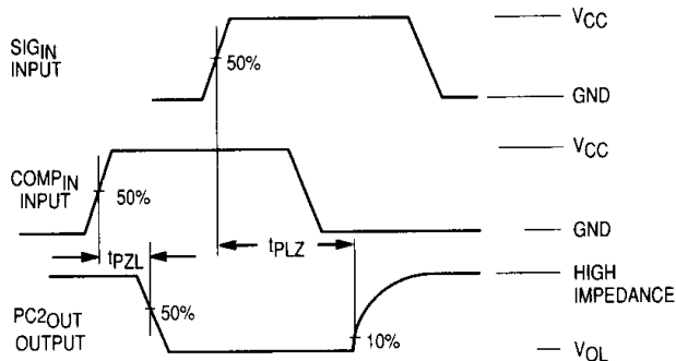
Figure 3. Switching Waveforms
