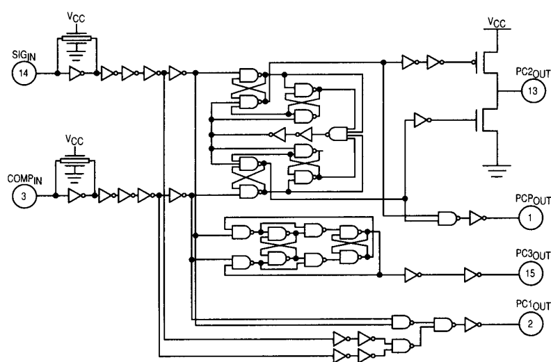
Figure 6. Logic Diagram for Phase Comparators
