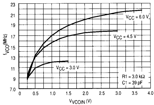
Figure 12A. VCO Frequency ( f_{VCO} ) as a Function of the VCO Input Voltage ( V_{VCO\_IN} )
