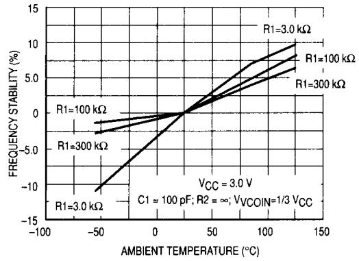
Figure 11A. Frequency Stability versus Ambient Temperature: V_{CC} = 3.0\text{ V}
