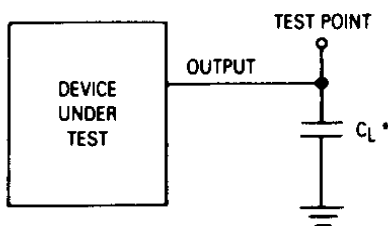
Figure 5. Test Circuit
