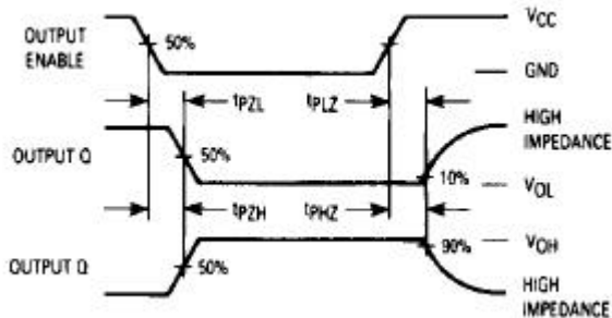
Figure 3. Switching Waveforms
