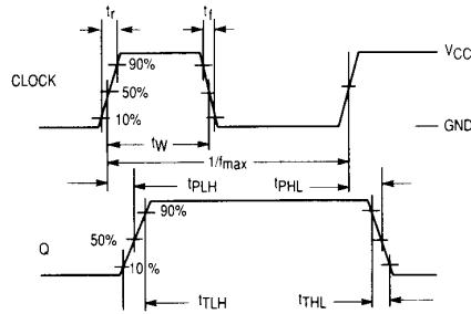
Figure 1. Switching Waveforms
