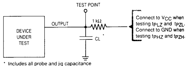
Figure 5. Test Circuit
