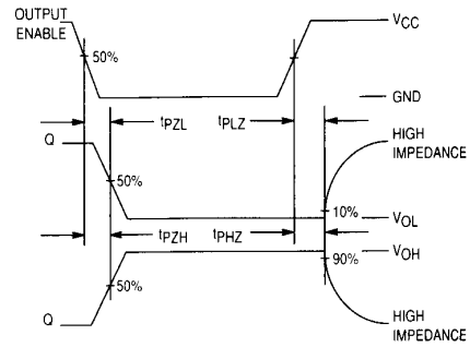
Figure 2. Switching Waveforms
