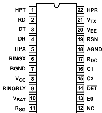
HC5515 (PDIP) TOP VIEW
