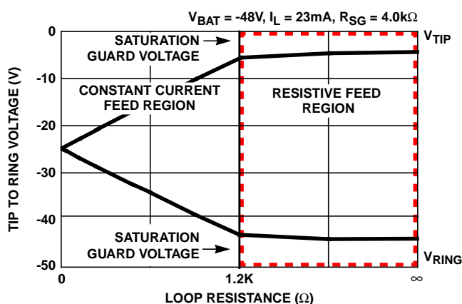
FIGURE 13. V_{TR} vs R_L
