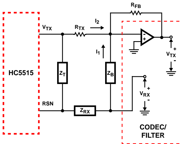
FIGURE 16. TRANSHYBRID CIRCUIT
