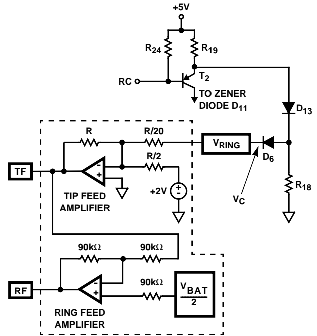
FIGURE 5. CENTERING VOLTAGE APPLICATION CIRCUIT
