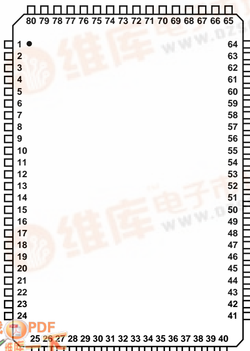
HC5519 (MQFP) TOP VIEW
