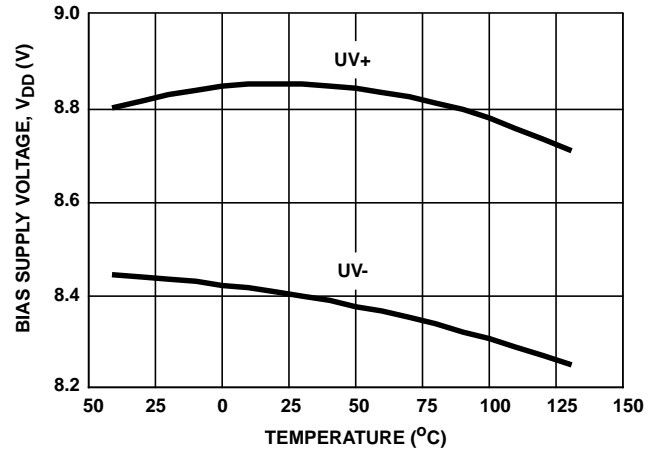
FIGURE 29. UNDERVOLTAGE LOCKOUT vs TEMPERATURE
