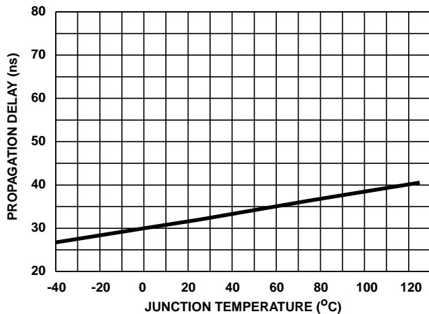
FIGURE 18. LOWER TURN-OFF PROPAGATION DELAY T_{LPLH} vs TEMPERATURE
