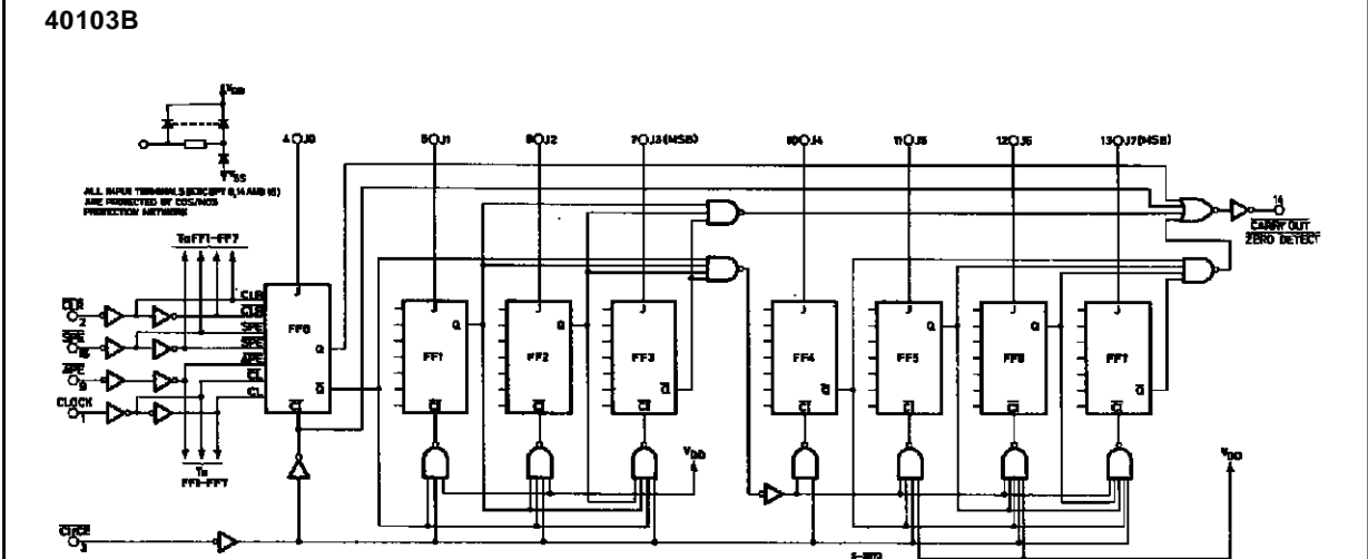
Detail logic diagram for flip-flops, FF0-FF7 used in logic diagrams for 40102B and 40103B.
