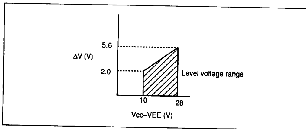
Figure 7 Relation between V_{CC} - V_{EE} and \Delta V
