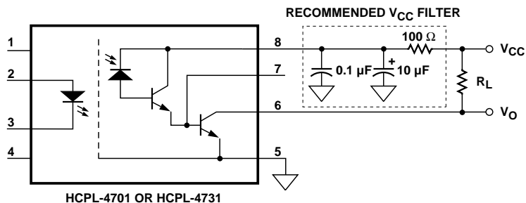
Figure 11. Typical Optical Isolation Used for Power-Loss Indication and Regulation Signal Feedback.
